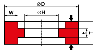
9 - D × T × H
