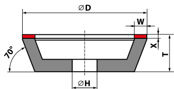
11A2 - D × T-X × W × X × H
