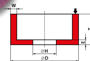
6 - D × T × H - W...E...
