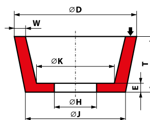
11 - D/J x T x H - W...E...K...
