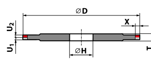
14AA1 - D \times U_1/U_2 \times X \times T \times H
