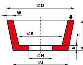
11 - D/J × T × H - W...E...K...
