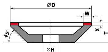
12A2-45 - D × T-X × W × X × H
